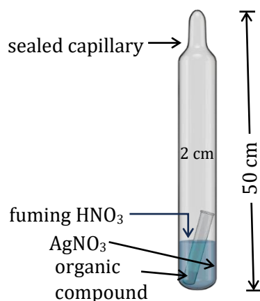
Figure : Carius method.
