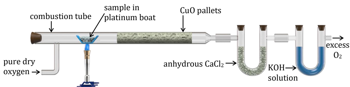
Figure : Estimation of carbon and hydrogen.
