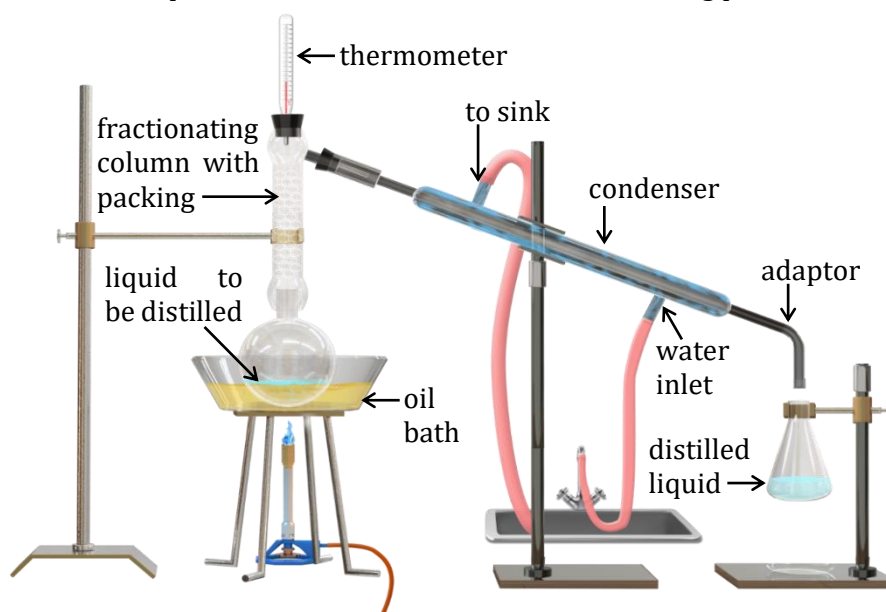
Figure : Fractional distillation.
