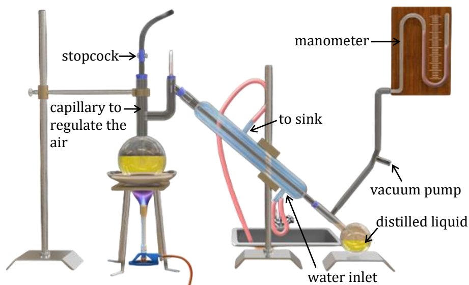
Figure : Distillation under reduced pressure.
