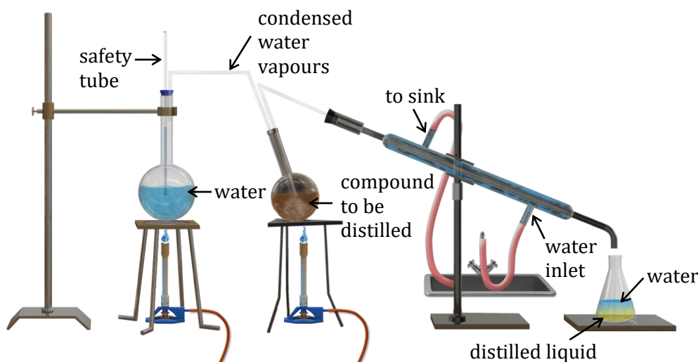
Figure : Steam distillation.
