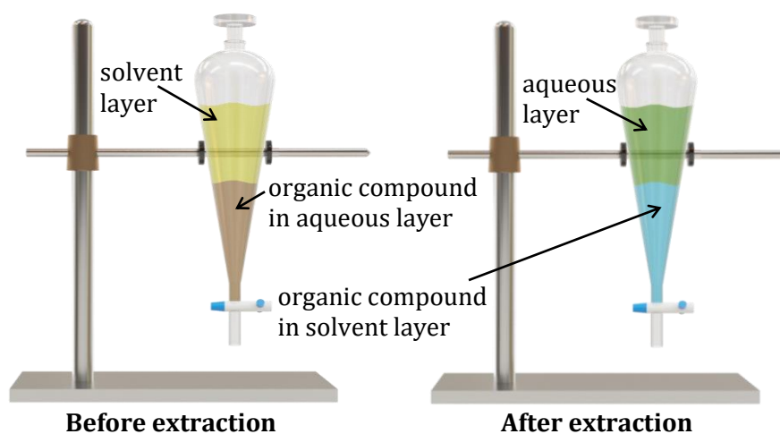
Figure : Differential extraction.
