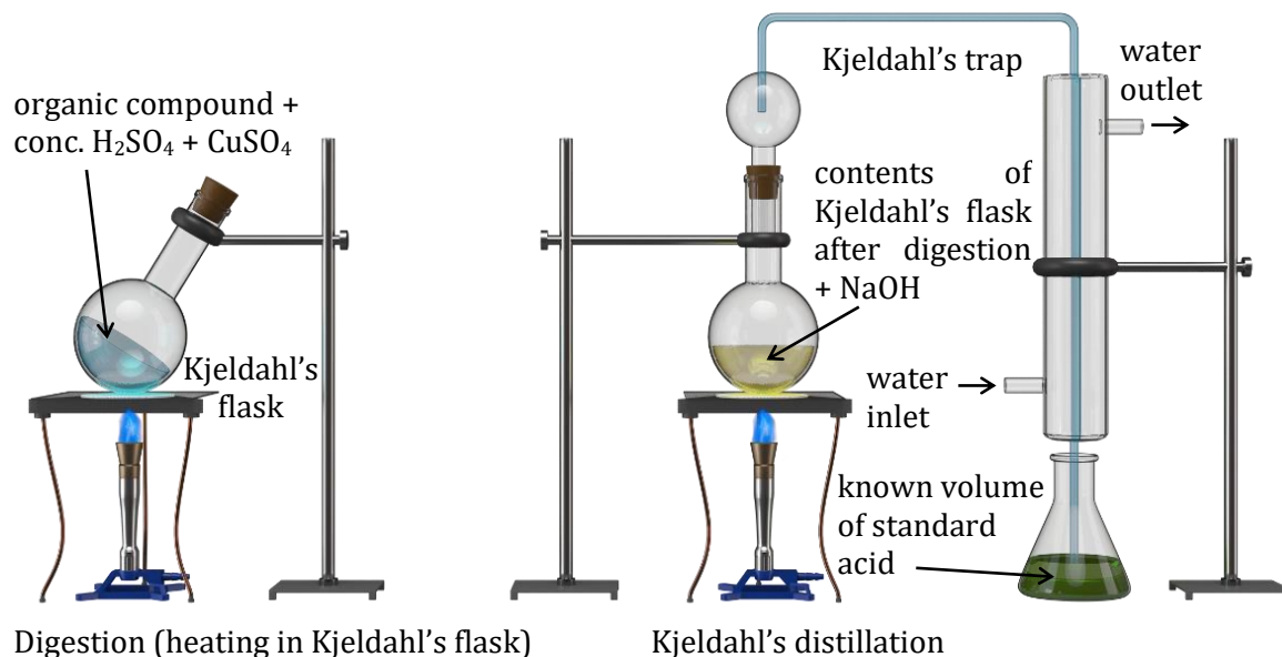
Figure : Kjeldahl method.
