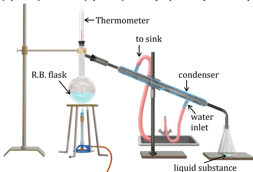
Figure : Simple distillation.
